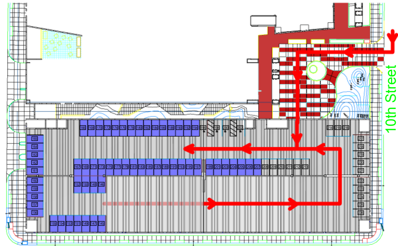
1 VISITOR PARKING PLAN - LEVEL P2 1" = 60'-0"
